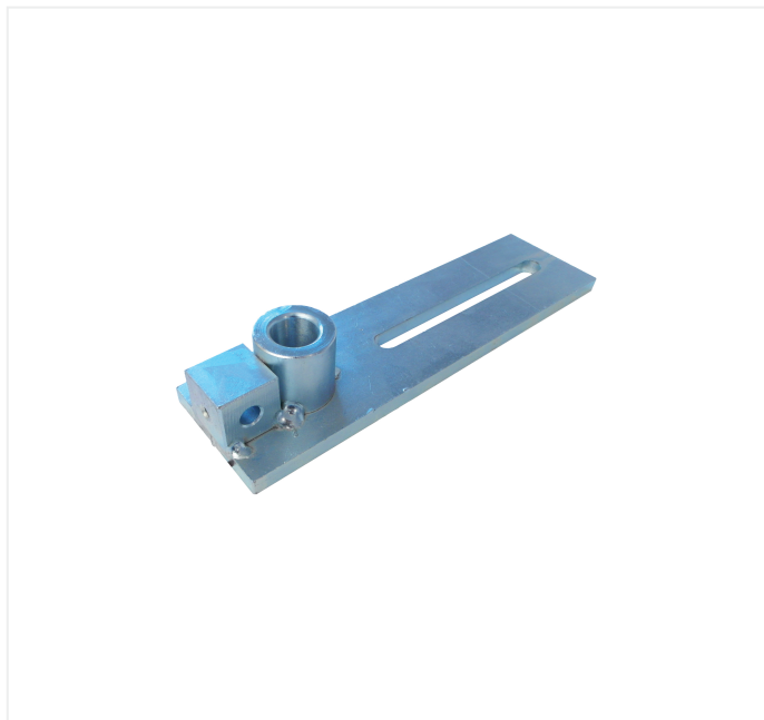
Support for drill jig
