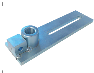
50018.3000 Support for drill jig Ø 30 mm
