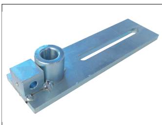
50018.4200 Support for drill jig Ø 42,5 mm
