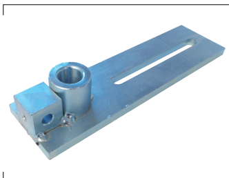
50018.2400 Support for drill jig Ø 24 mm
